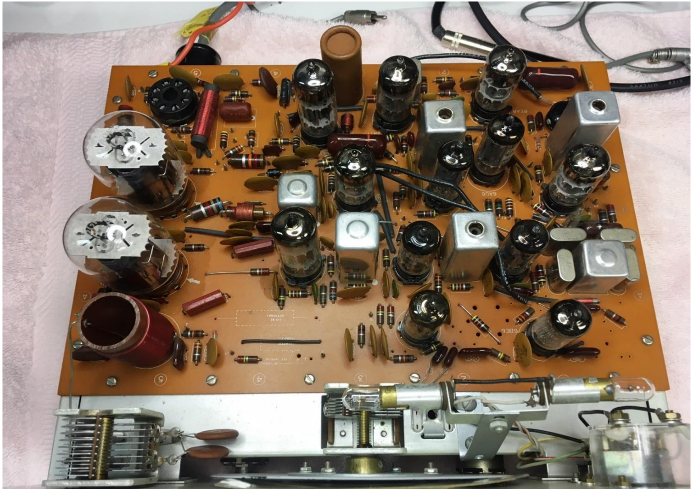
Heathkit HW-12 Chassis Top View
