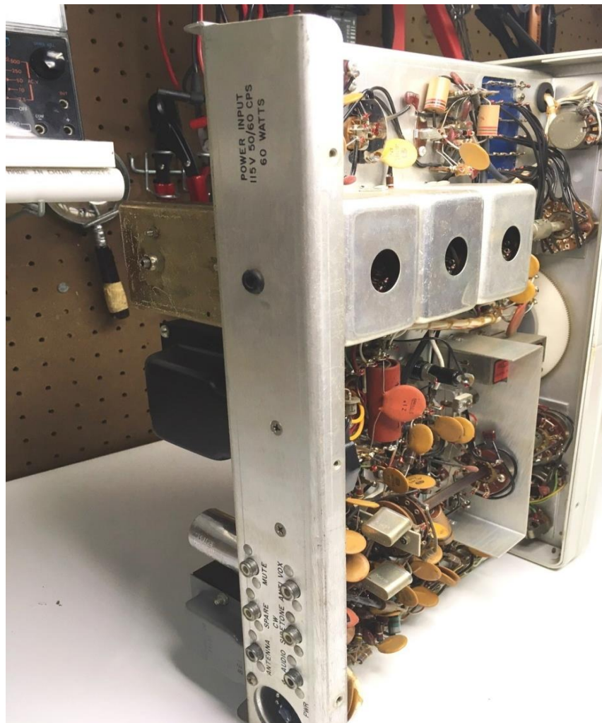
Collins 75S-3 Chassis Bottom Views
