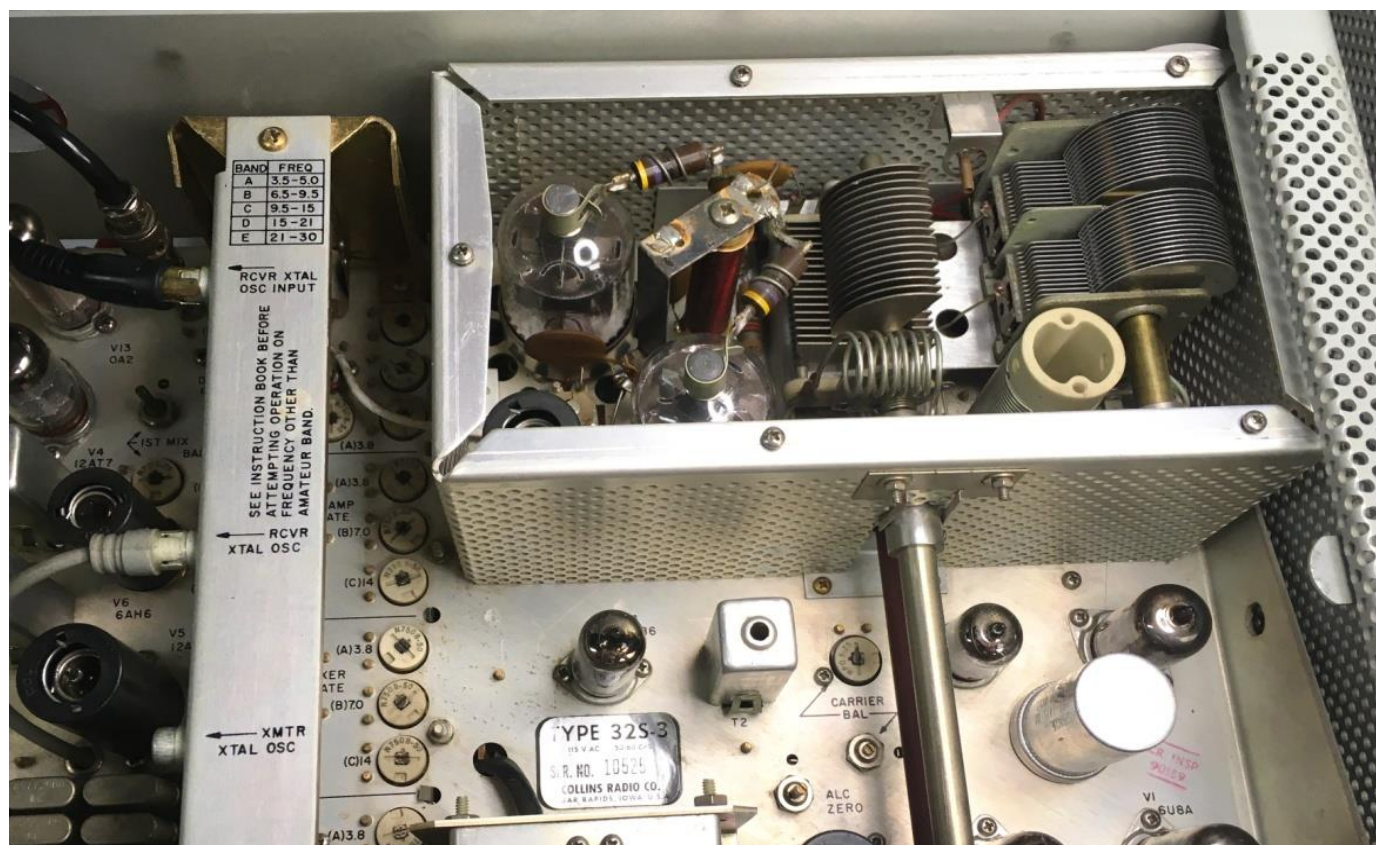
Collins 32S-3 Chassis Top Views
