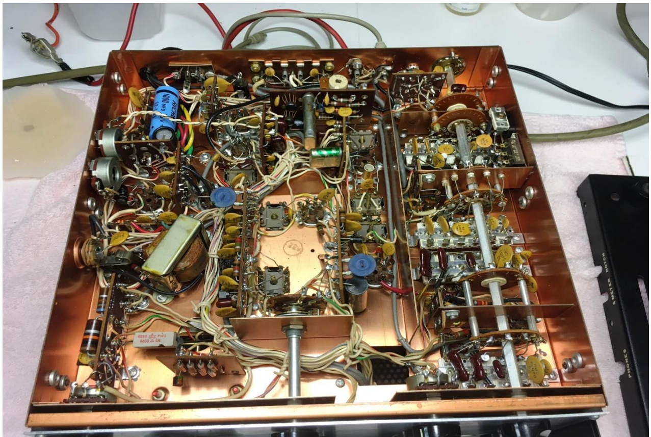
Drake R-4B Chassis Views
