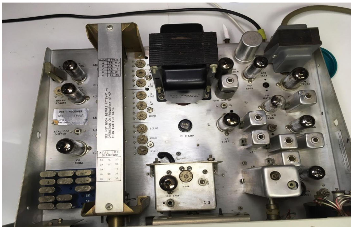
Collins 75S-3 Chassis Top View
