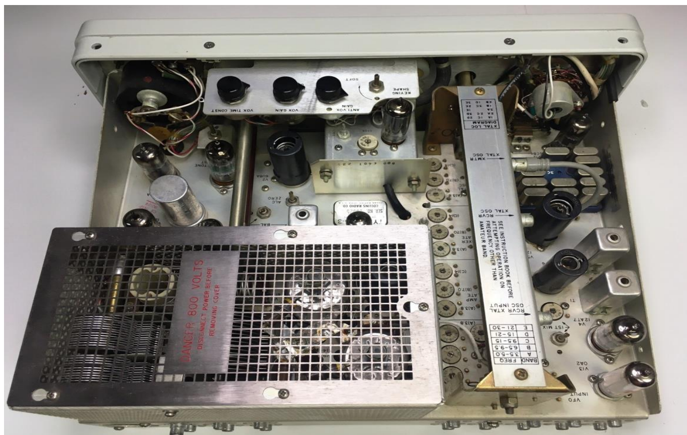
Collins 32S-3 Chassis Top Views
