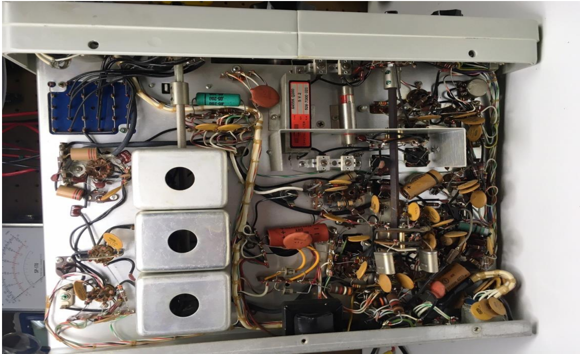
Collins 75S-3 Chassis Bottom Views
