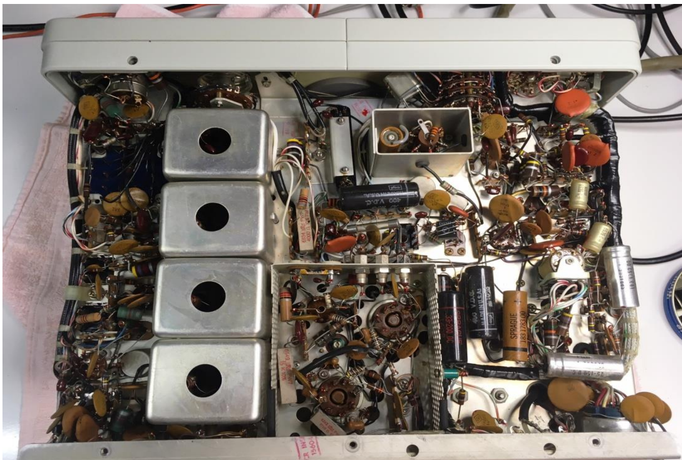
Collins 32S-3 Chassis Bottom and Rear View
